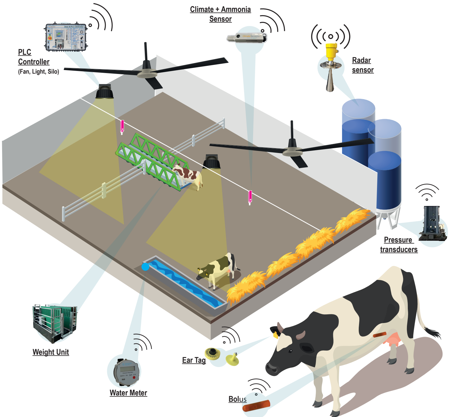
Lorawan Transmitters
